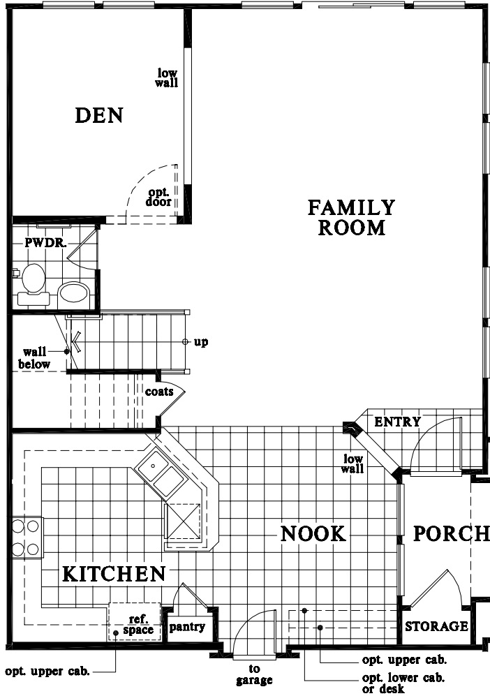
UNIT "E" FIRST FLOOR 1964 S.F.
