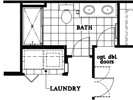
OPT. SHOWER AT BATH
